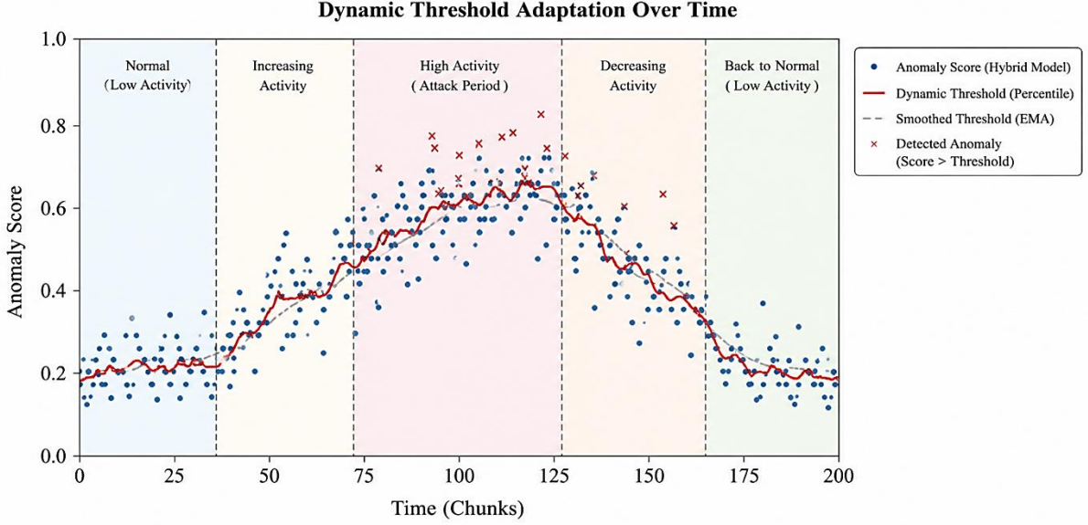
Figure 5: Dynamic threshold adaptation over time based on anomaly score distribution.
